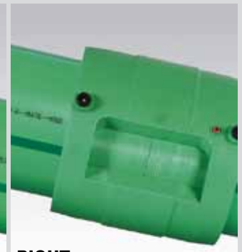
Push the second pipe - also peeled and cleaned - into the socket
